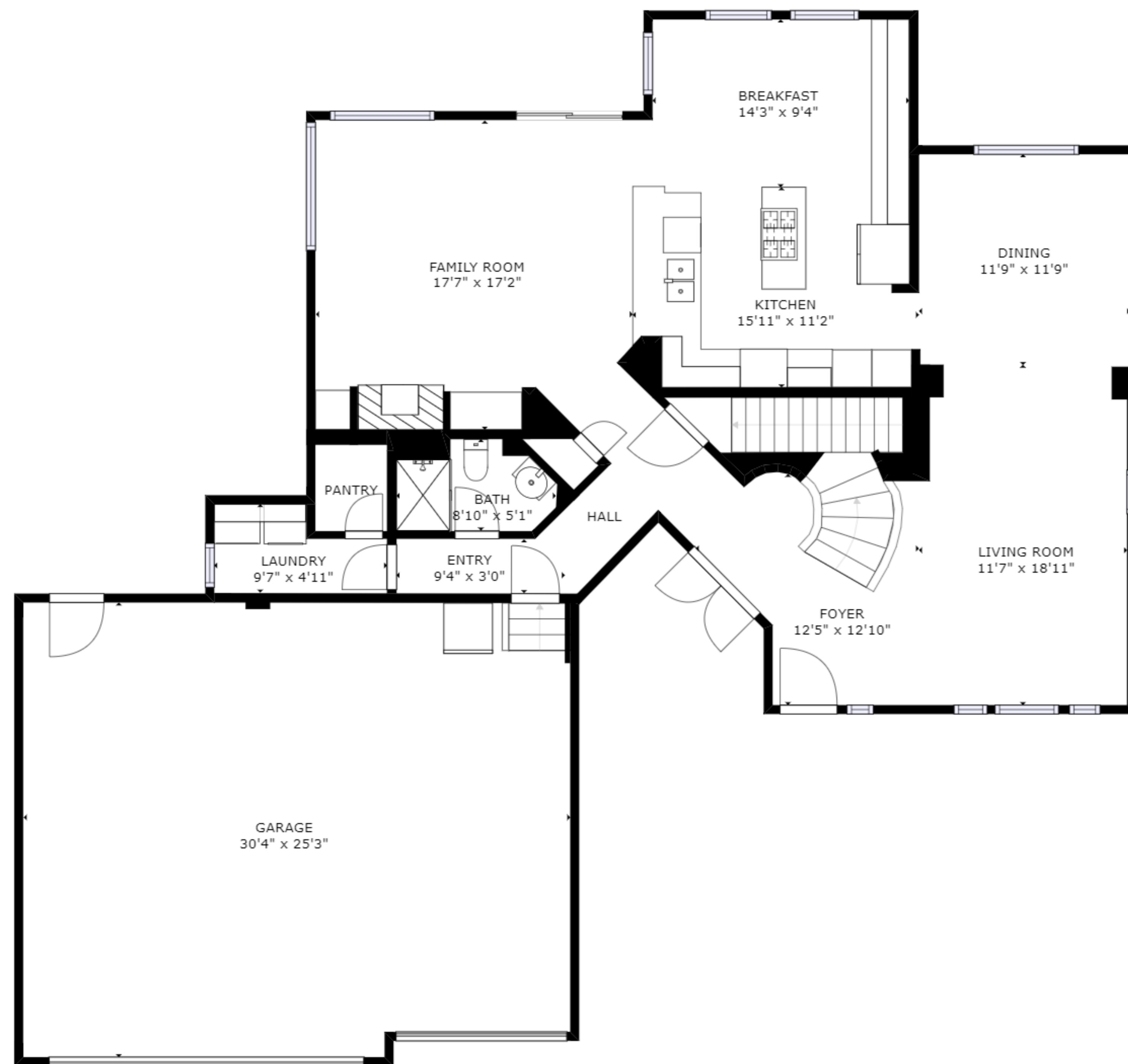
FLOOR 2
