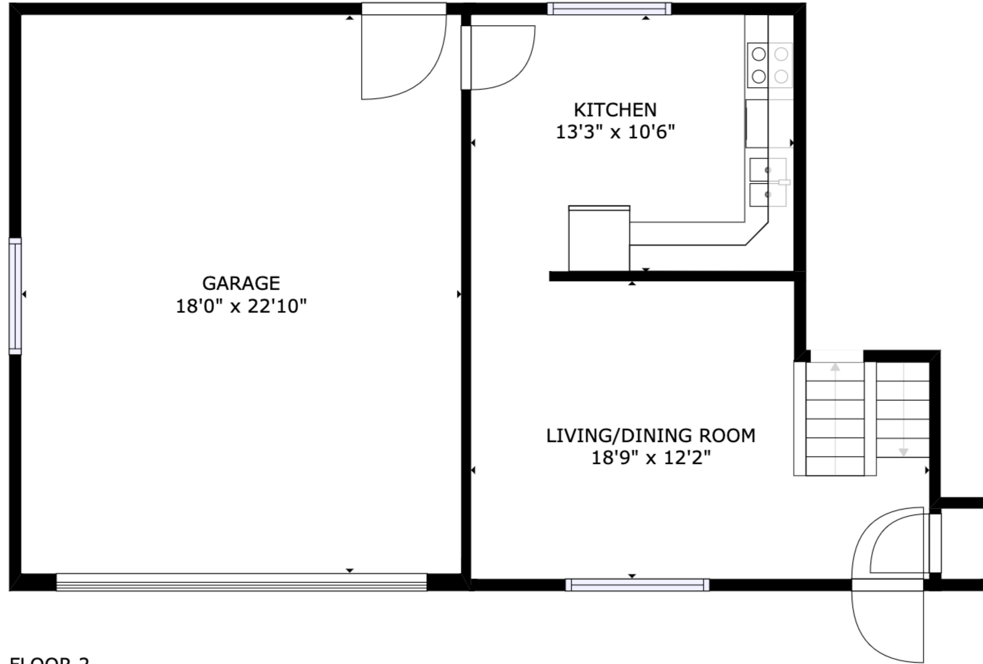
FLOOR 2
